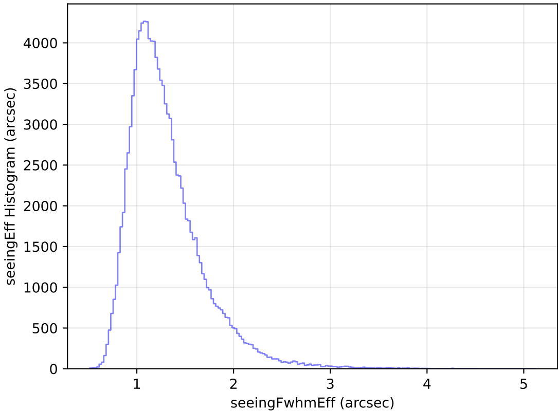
roll_pause_mjdp120_v3.4_10yrs WFD u band: seeingEff Histogram
