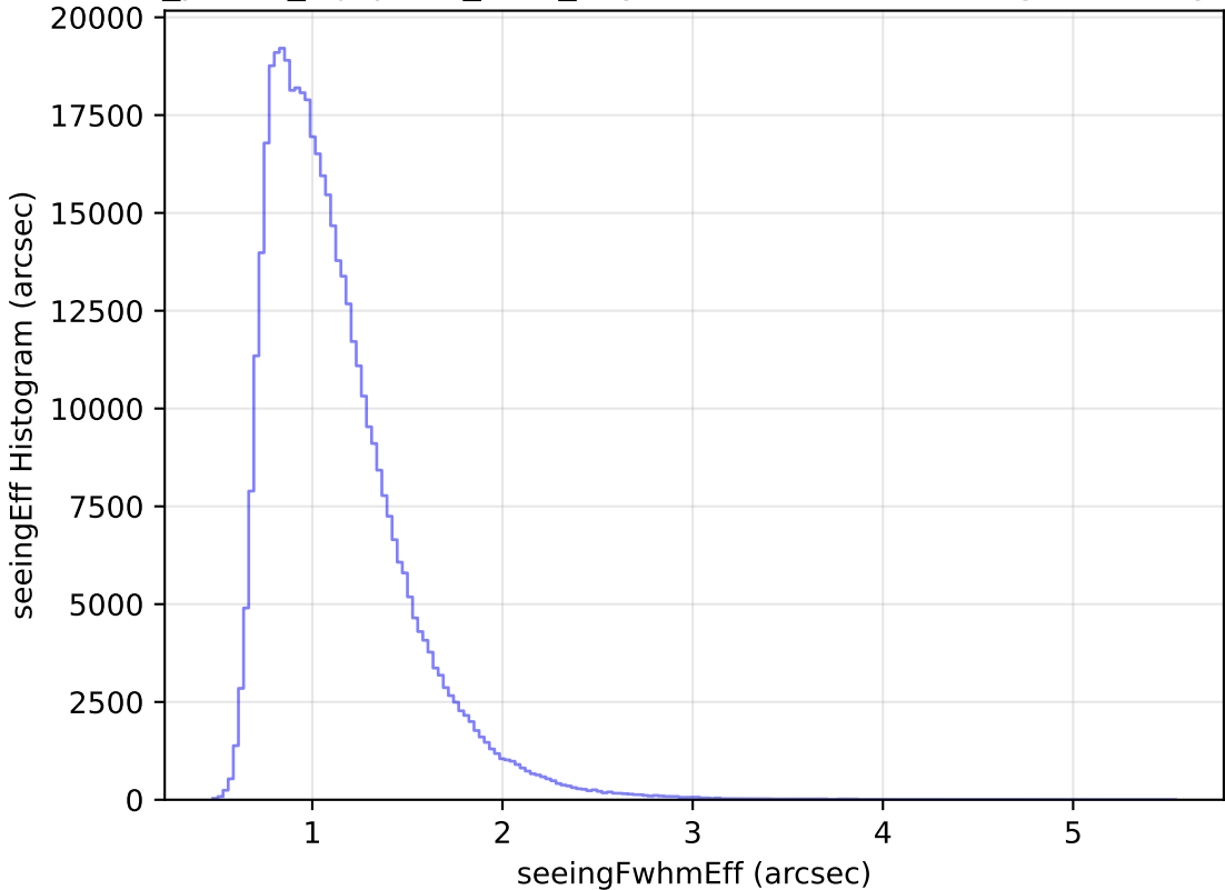
roll_pause_mjdp120_v3.4_10yrs WFD r band: seeingEff Histogram
