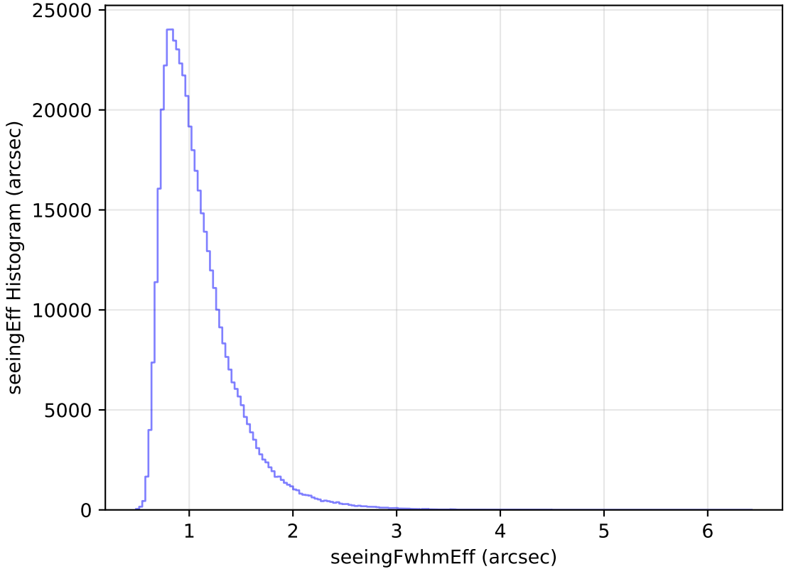
roll_pause_mjdp120_v3.4_10yrs WFD i band: seeingEff Histogram
