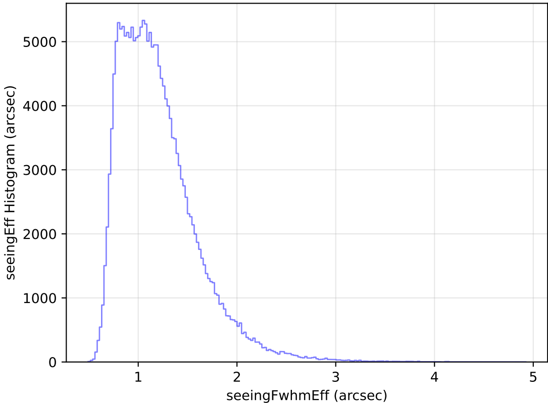
roll_pause_mjdp120_v3.4_10yrs WFD g band: seeingEff Histogram
