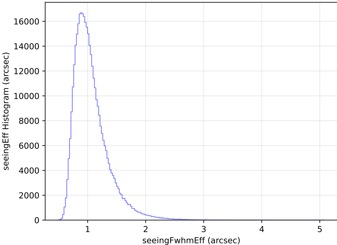
roll_pause_mjdp120_v3.4_10yrs All sky y band: seeingEff Histogram
