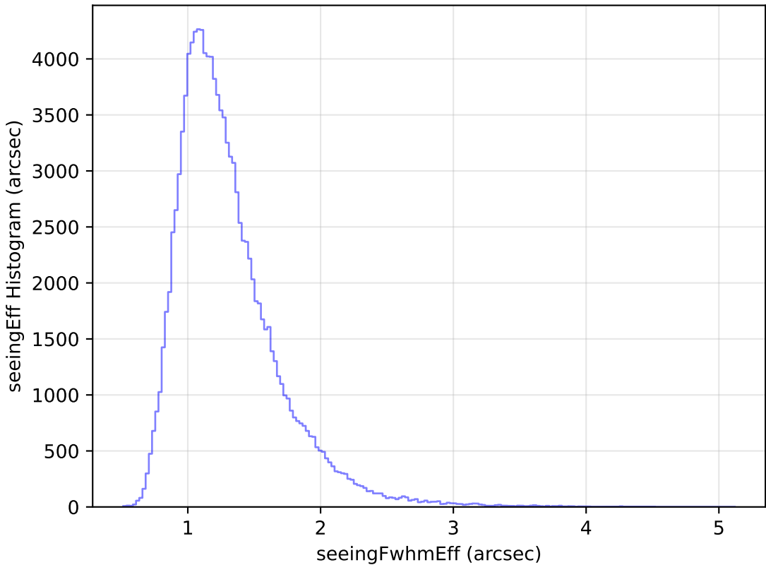
roll_pause_mjdp120_v3.4_10yrs All sky u band: seeingEff Histogram
