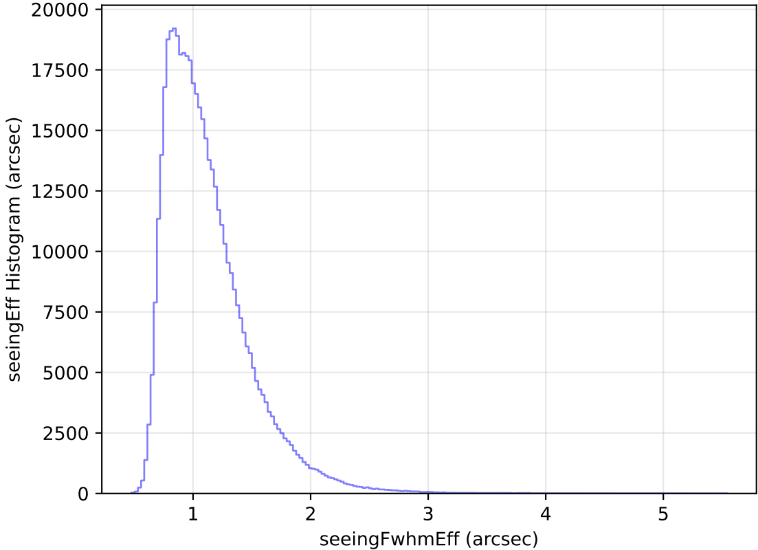
roll_pause_mjdp120_v3.4_10yrs All sky r band: seeingEff Histogram
