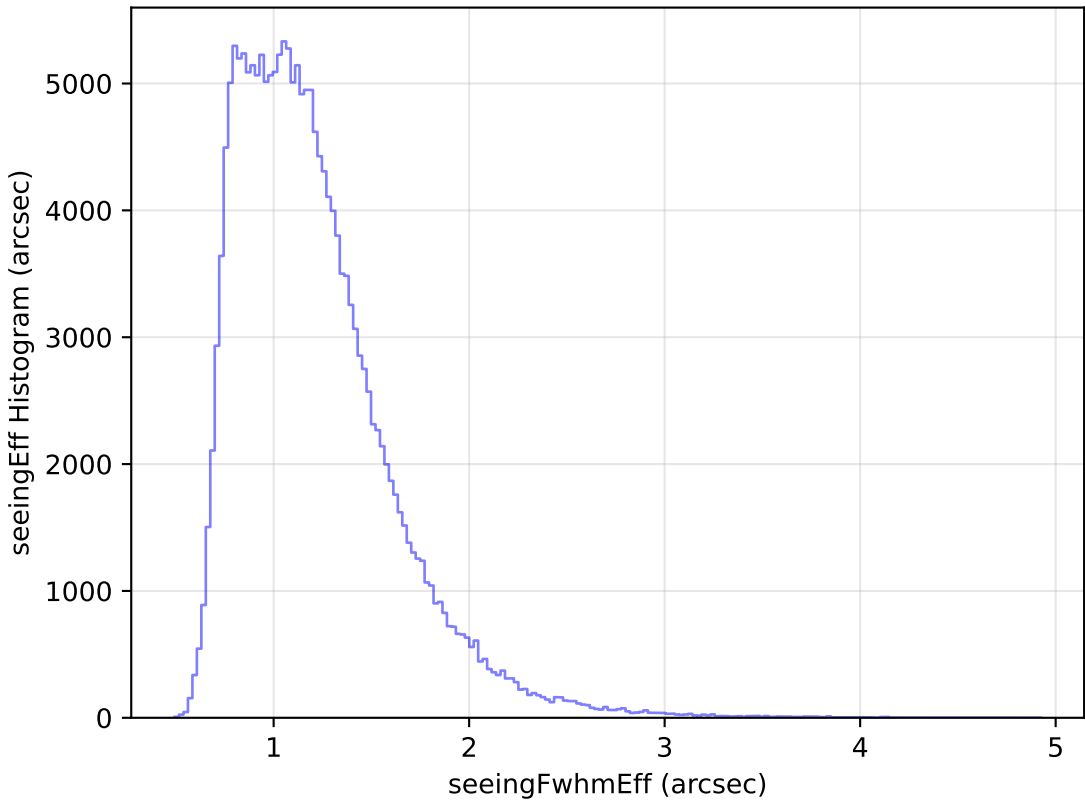
roll_pause_mjdp120_v3.4_10yrs All sky g band: seeingEff Histogram
