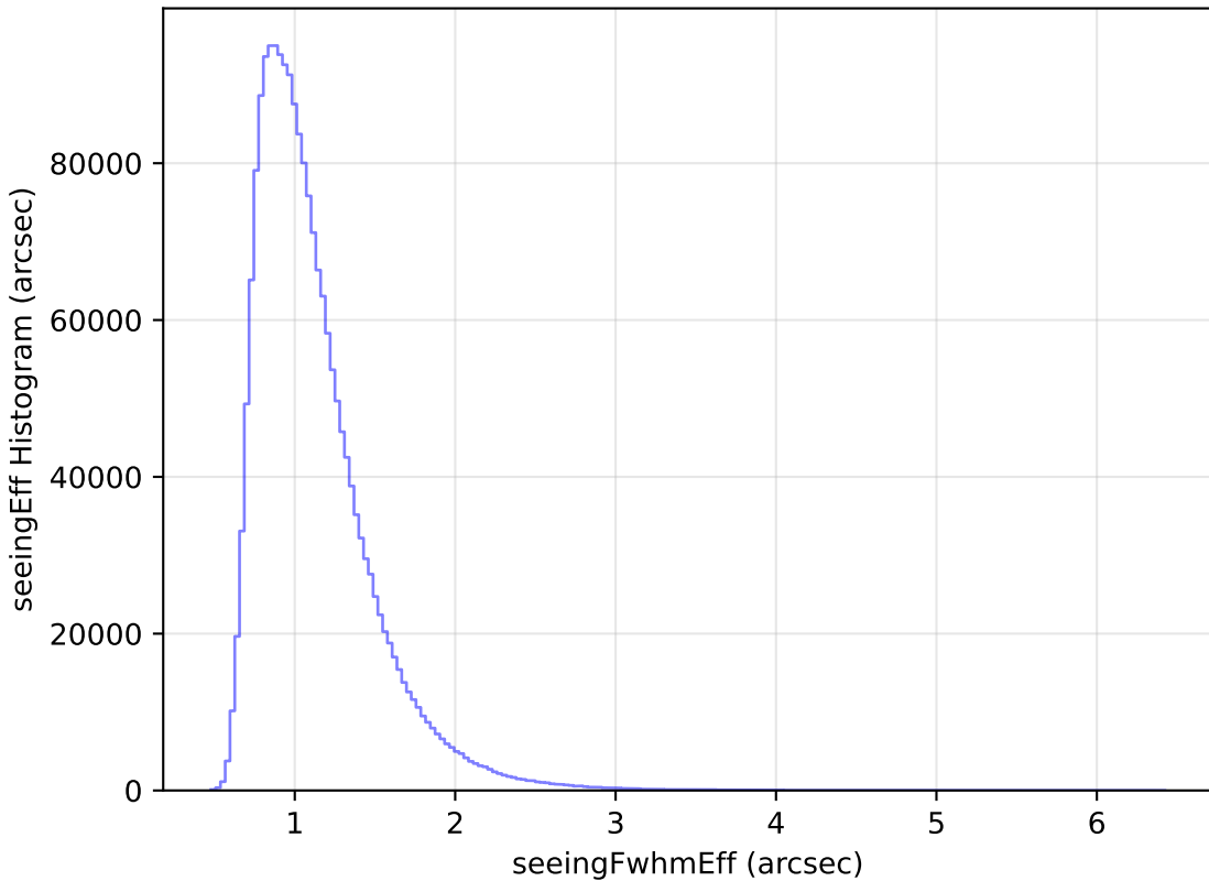
roll_pause_mjdp120_v3.4_10yrs All sky all bands: seeingEff Histogram
