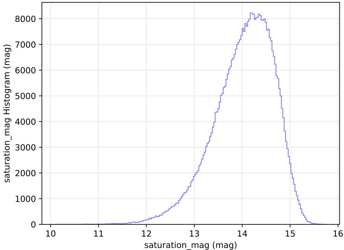
roll_pause_mjdp120_v3.4_10yrs WFD z band: saturation_mag Histogram
