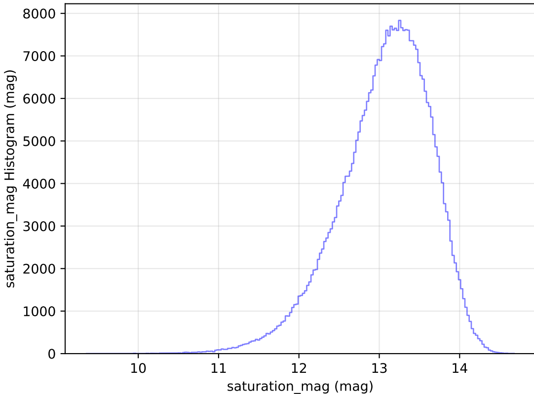
roll_pause_mjdp120_v3.4_10yrs WFD y band: saturation_mag Histogram
