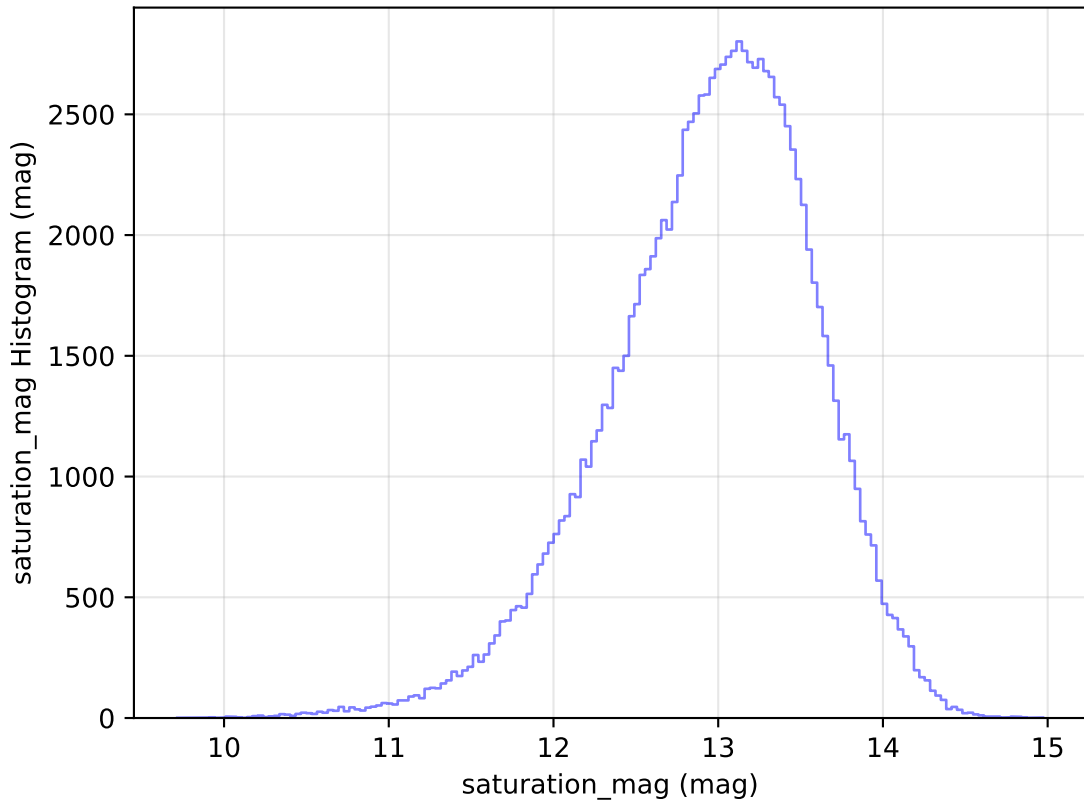
roll_pause_mjdp120_v3.4_10yrs WFD u band: saturation_mag Histogram
