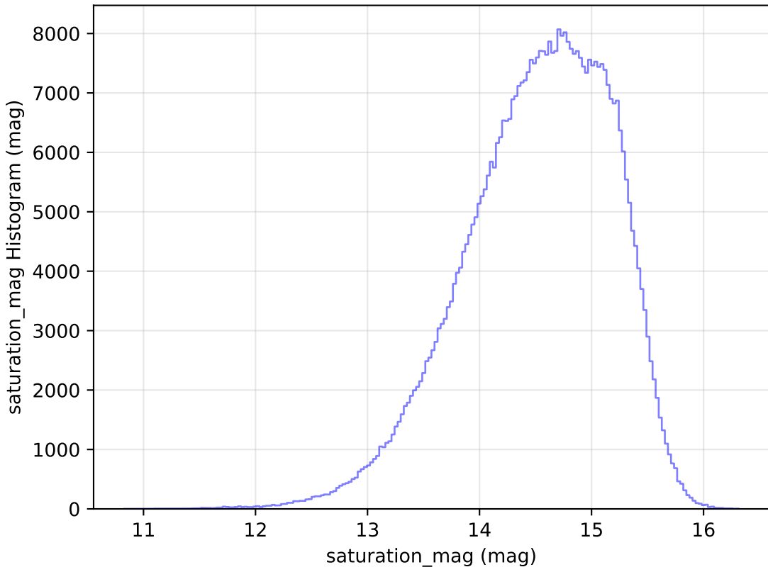
roll_pause_mjdp120_v3.4_10yrs WFD r band: saturation_mag Histogram
