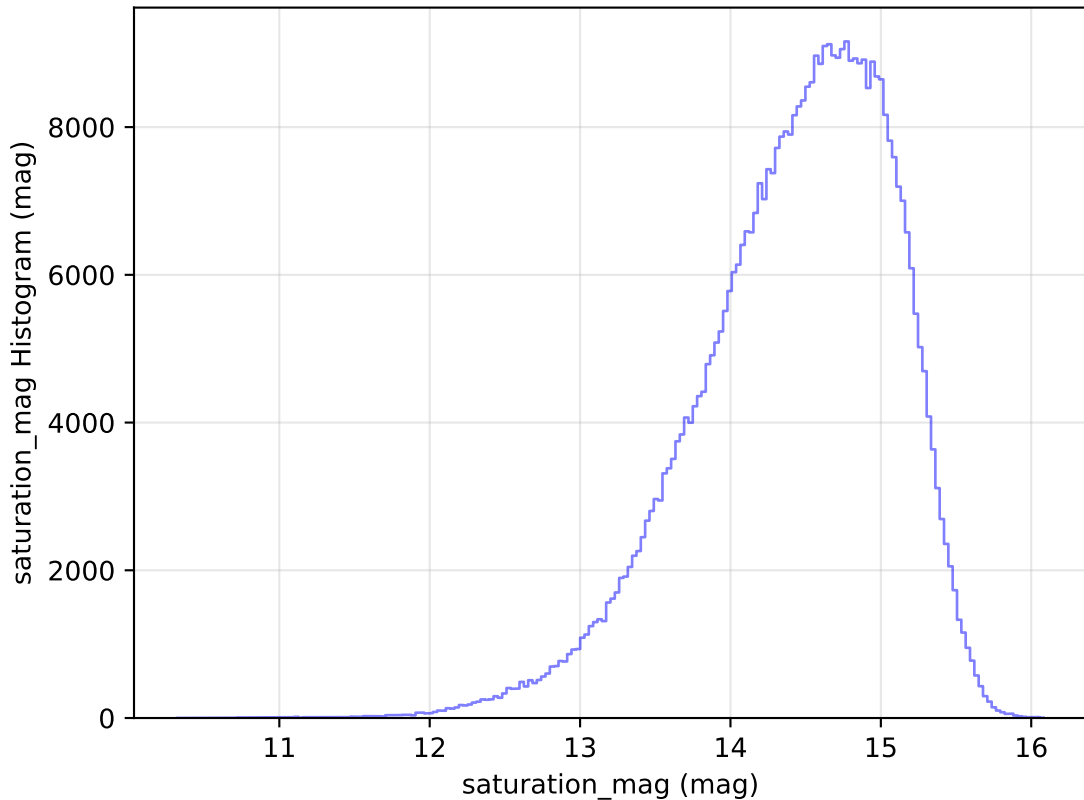
roll_pause_mjdp120_v3.4_10yrs WFD i band: saturation_mag Histogram
