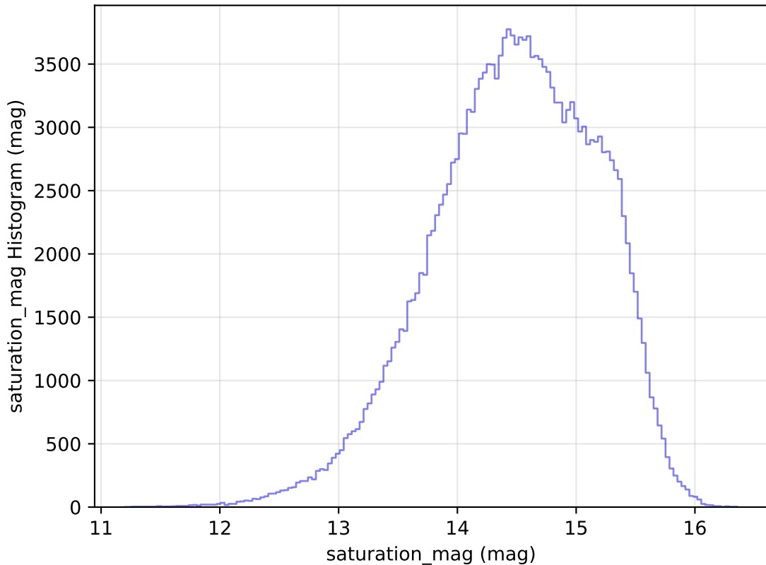
roll_pause_mjdp120_v3.4_10yrs WFD g band: saturation_mag Histogram
