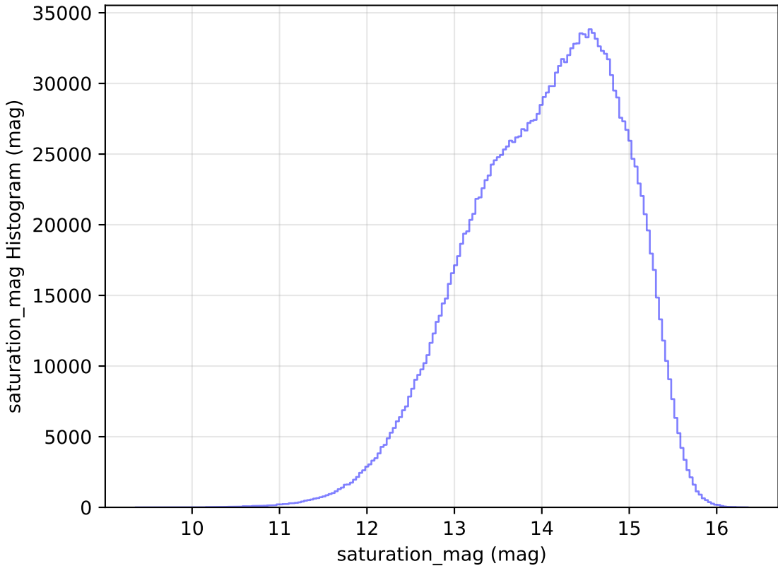
roll_pause_mjdp120_v3.4_10yrs WFD all bands: saturation_mag Histogram
