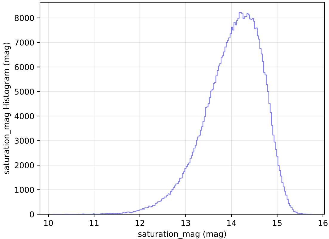
roll_pause_mjdp120_v3.4_10yrs All sky z band: saturation_mag Histogram
