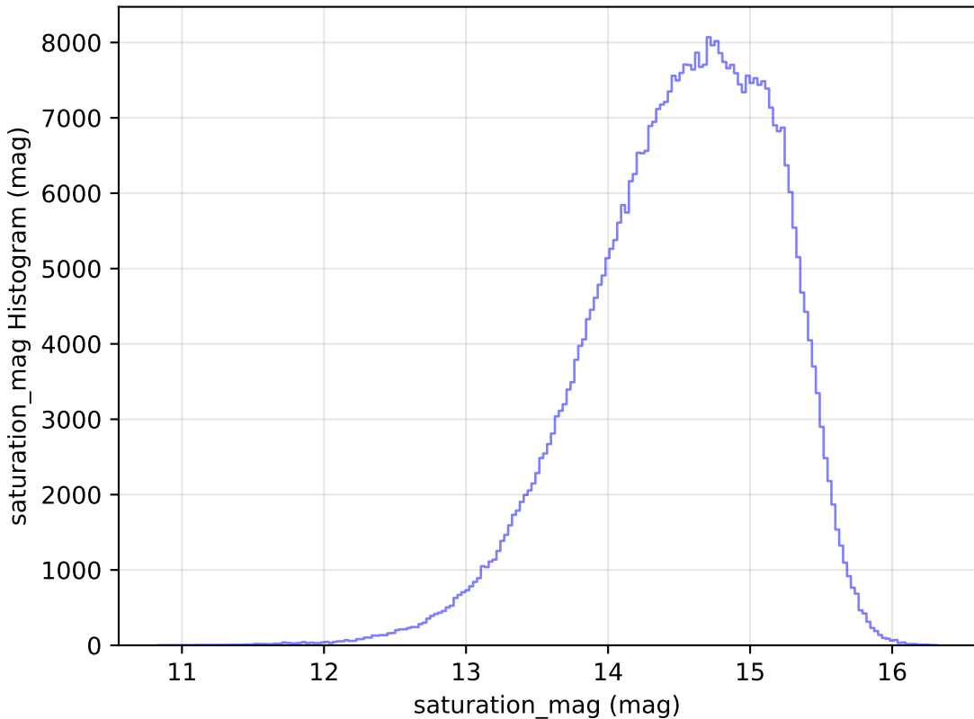
roll_pause_mjdp120_v3.4_10yrs All sky r band: saturation_mag Histogram
