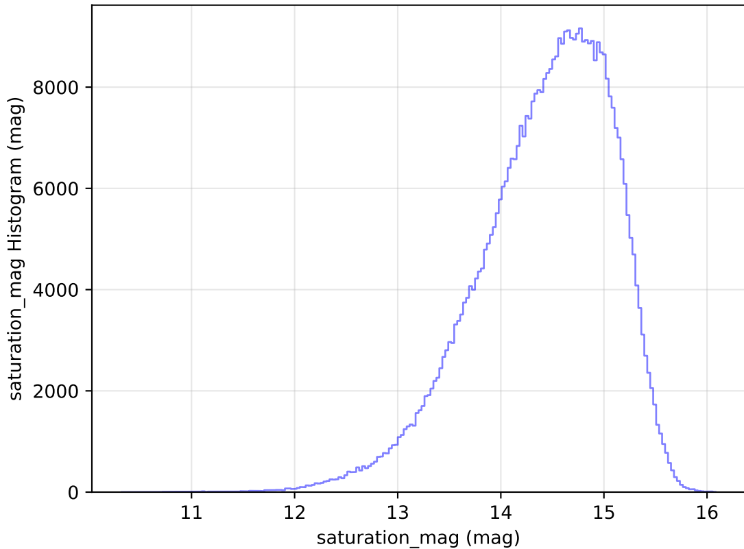
roll_pause_mjdp120_v3.4_10yrs All sky i band: saturation_mag Histogram
