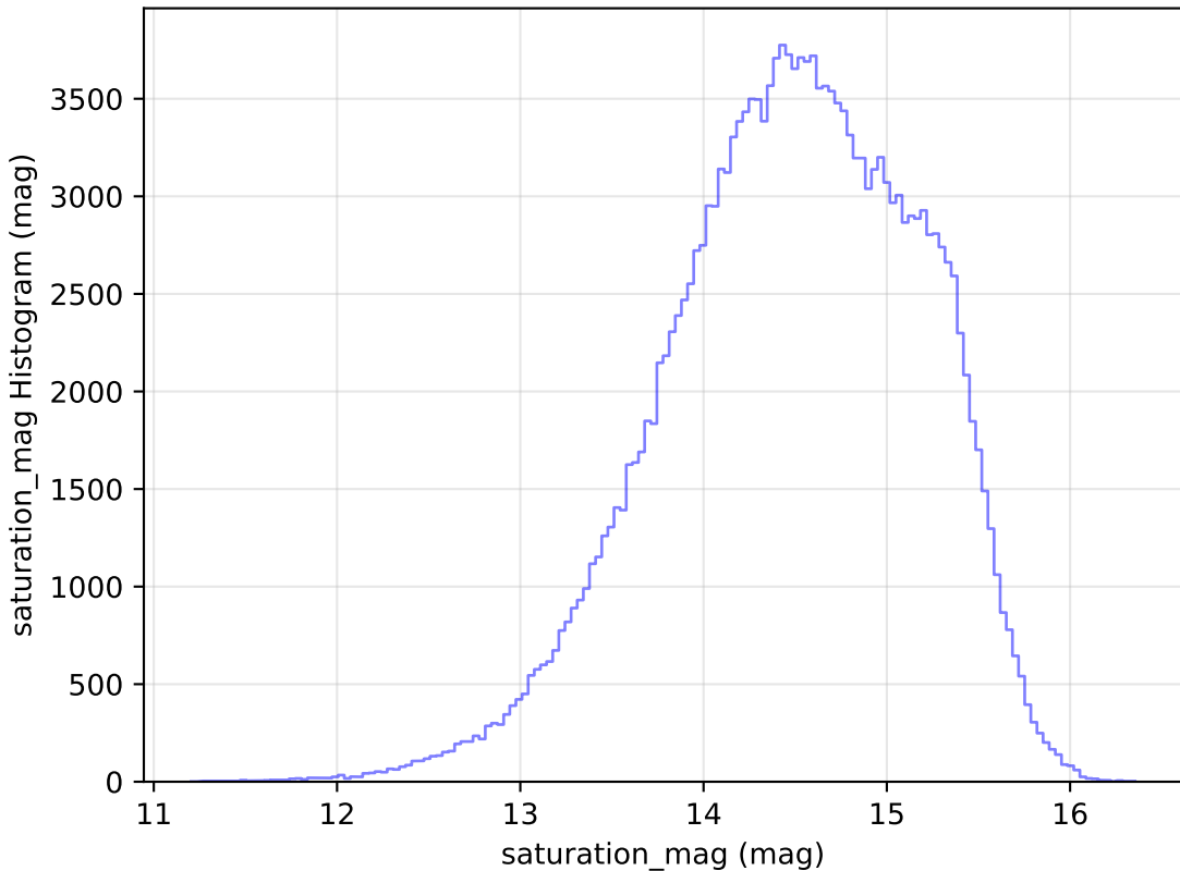
roll_pause_mjdp120_v3.4_10yrs All sky g band: saturation_mag Histogram
