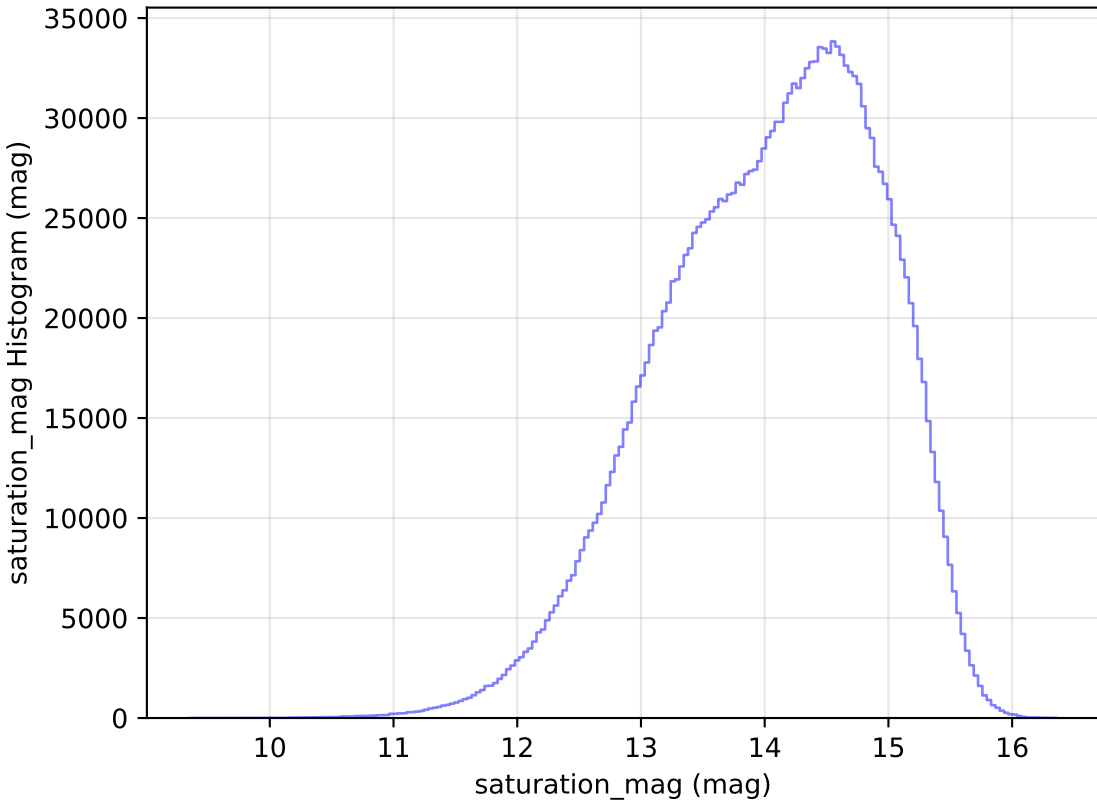
roll_pause_mjdp120_v3.4_10yrs All sky all bands: saturation_mag Histogram
