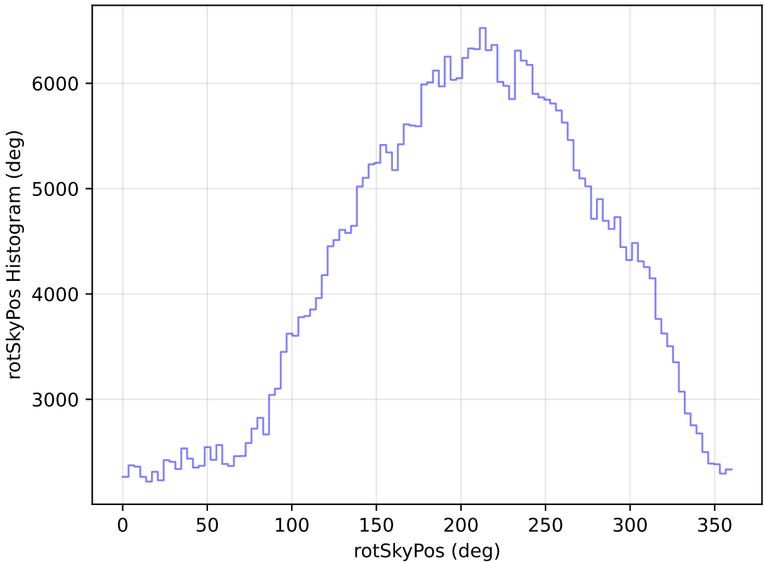
roll_pause_mjdp120_v3.4_10yrs WFD z band: rotSkyPos Histogram
