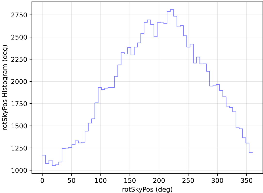
roll_pause_mjdp120_v3.4_10yrs WFD u band: rotSkyPos Histogram
