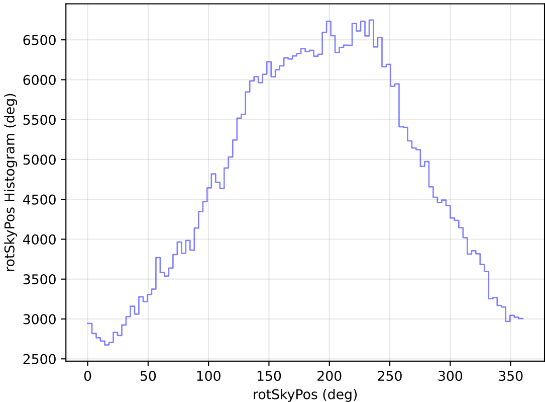
roll_pause_mjdp120_v3.4_10yrs WFD r band: rotSkyPos Histogram
