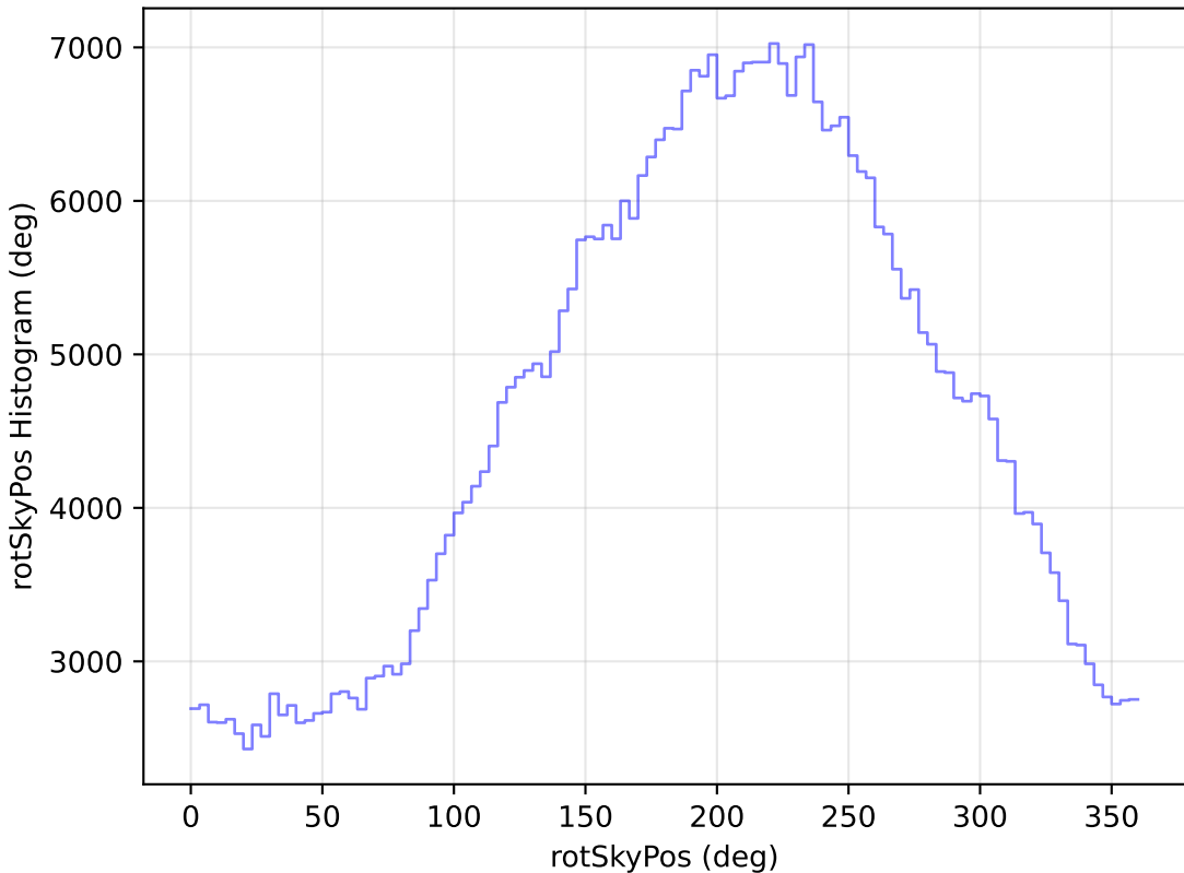
roll_pause_mjdp120_v3.4_10yrs WFD i band: rotSkyPos Histogram
