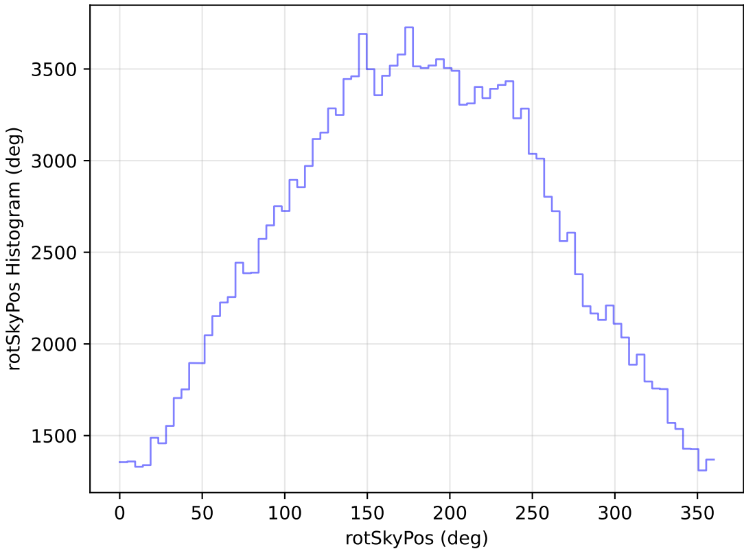
roll_pause_mjdp120_v3.4_10yrs WFD g band: rotSkyPos Histogram
