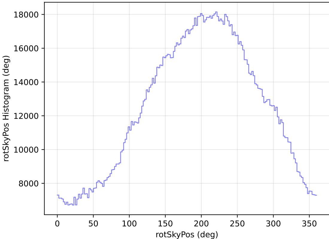
roll_pause_mjdp120_v3.4_10yrs WFD all bands: rotSkyPos Histogram
