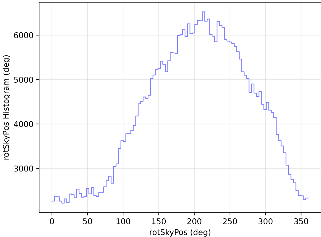
roll_pause_mjdp120_v3.4_10yrs All sky z band: rotSkyPos Histogram
