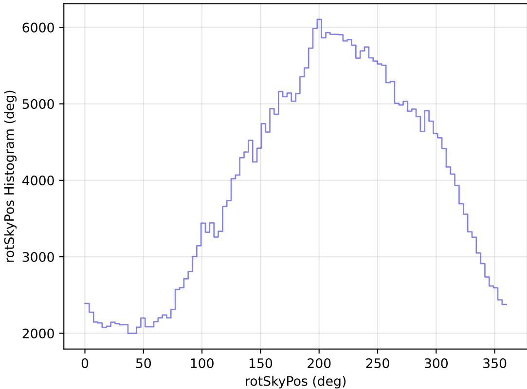
roll_pause_mjdp120_v3.4_10yrs All sky y band: rotSkyPos Histogram
