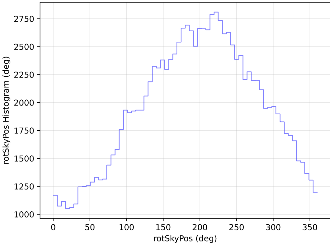
roll_pause_mjdp120_v3.4_10yrs All sky u band: rotSkyPos Histogram
