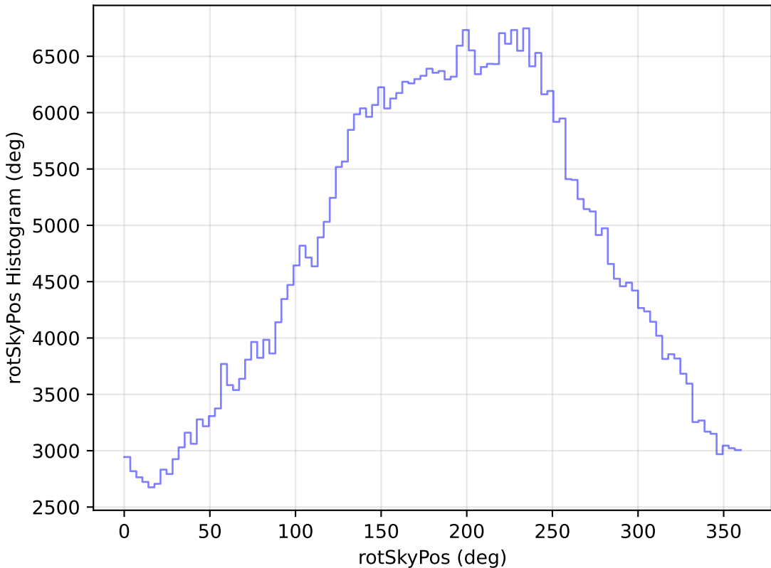
roll_pause_mjdp120_v3.4_10yrs All sky r band: rotSkyPos Histogram
