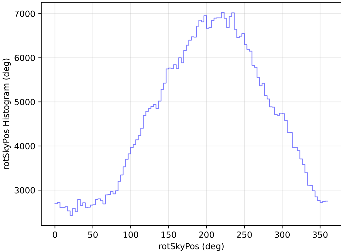
roll_pause_mjdp120_v3.4_10yrs All sky i band: rotSkyPos Histogram
