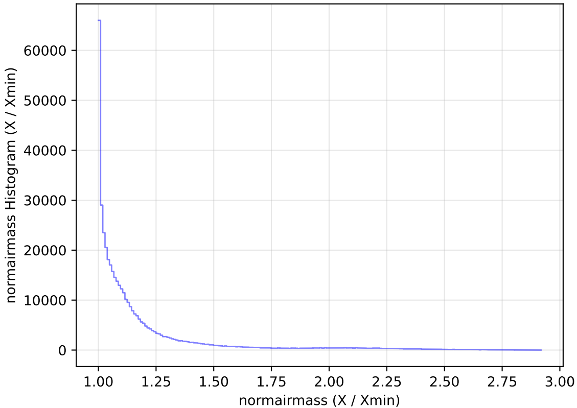
roll_pause_mjdp120_v3.4_10yrs WFD z band: normairmass Histogram
