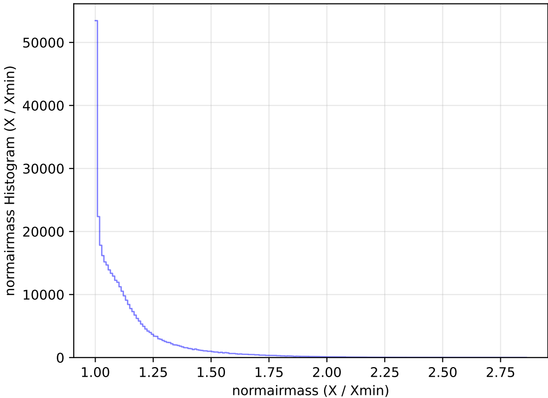
roll_pause_mjdp120_v3.4_10yrs WFD y band: normairmass Histogram
