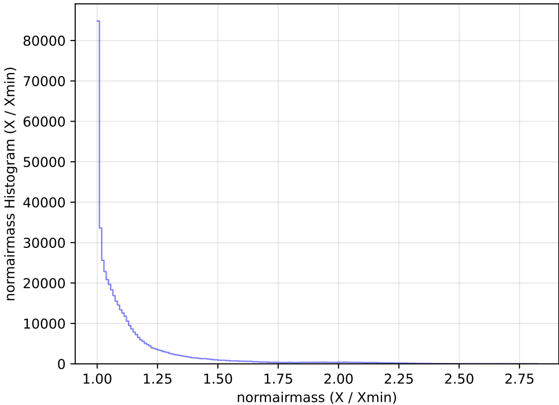
roll_pause_mjdp120_v3.4_10yrs WFD r band: normairmass Histogram
