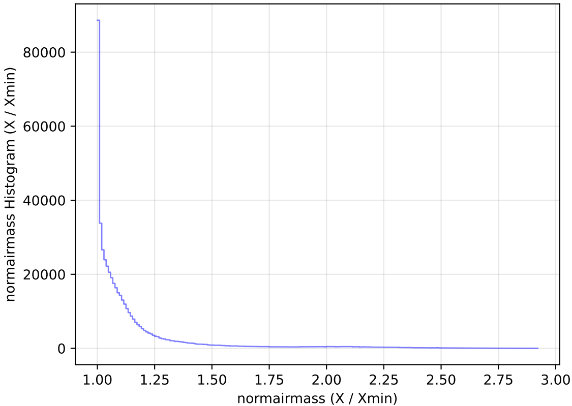
roll_pause_mjdp120_v3.4_10yrs WFD i band: normairmass Histogram
