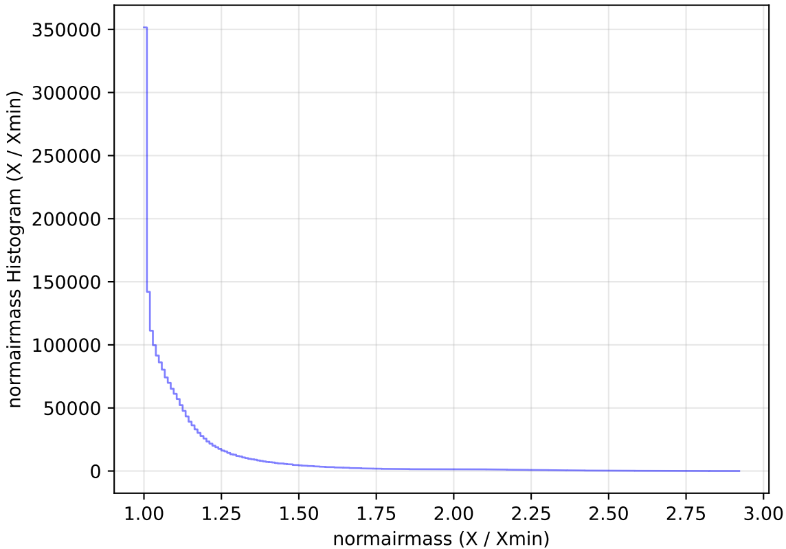
roll_pause_mjdp120_v3.4_10yrs WFD all bands: normairmass Histogram
