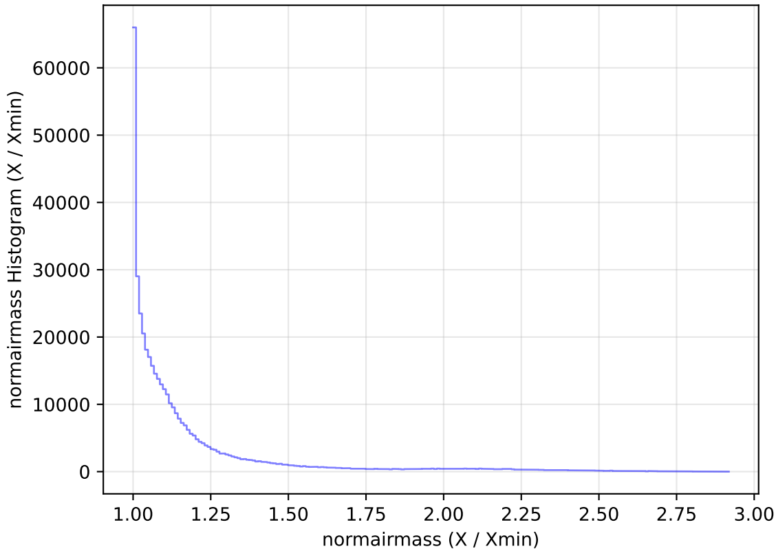
roll_pause_mjdp120_v3.4_10yrs All sky z band: normairmass Histogram
