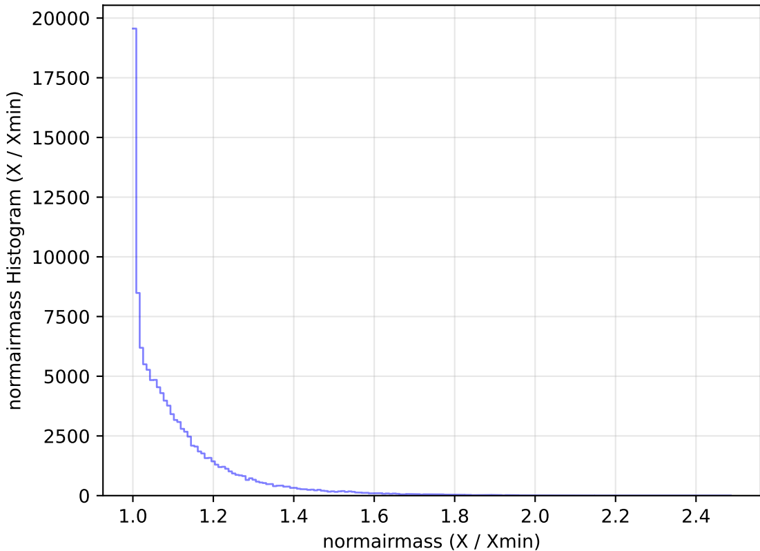
roll_pause_mjdp120_v3.4_10yrs All sky u band: normairmass Histogram
