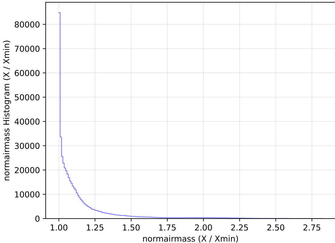
roll_pause_mjdp120_v3.4_10yrs All sky r band: normairmass Histogram
