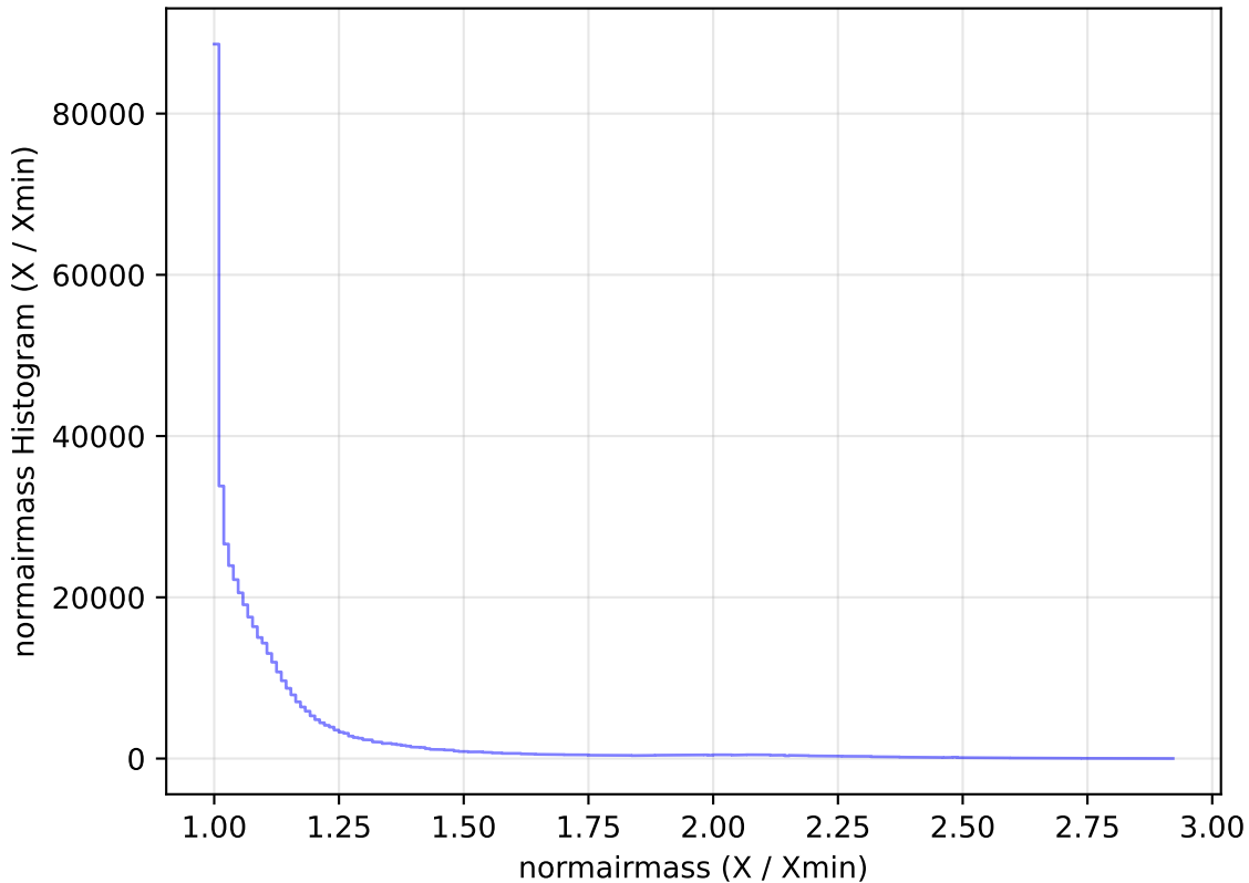
roll_pause_mjdp120_v3.4_10yrs All sky i band: normairmass Histogram
