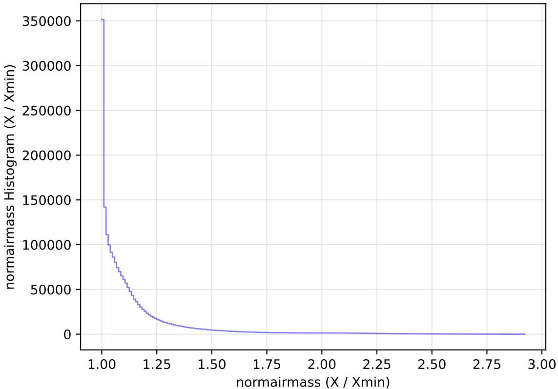
roll_pause_mjdp120_v3.4_10yrs All sky all bands: normairmass Histogram
