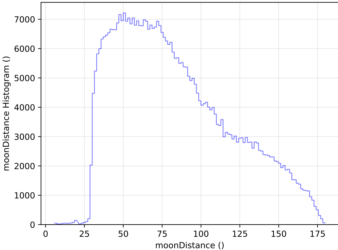
roll_pause_mjdp120_v3.4_10yrs WFD z band: moonDistance Histogram
