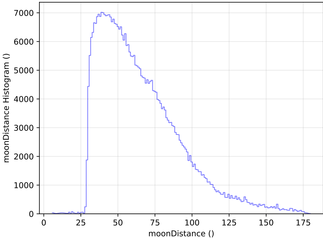
roll_pause_mjdp120_v3.4_10yrs WFD y band: moonDistance Histogram
