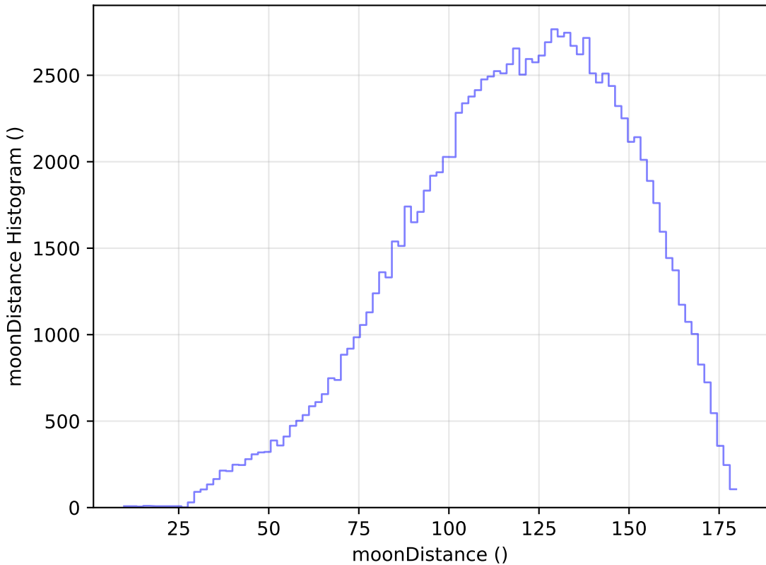
roll_pause_mjdp120_v3.4_10yrs WFD u band: moonDistance Histogram
