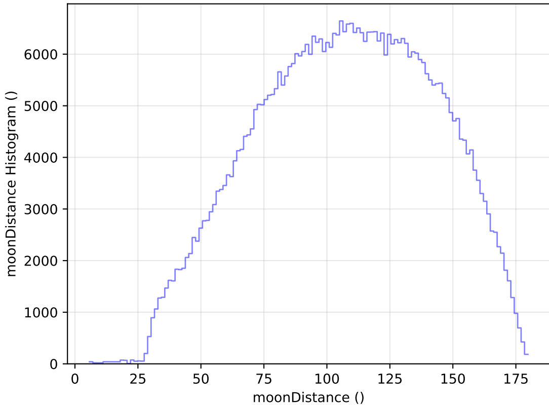
roll_pause_mjdp120_v3.4_10yrs WFD r band: moonDistance Histogram
