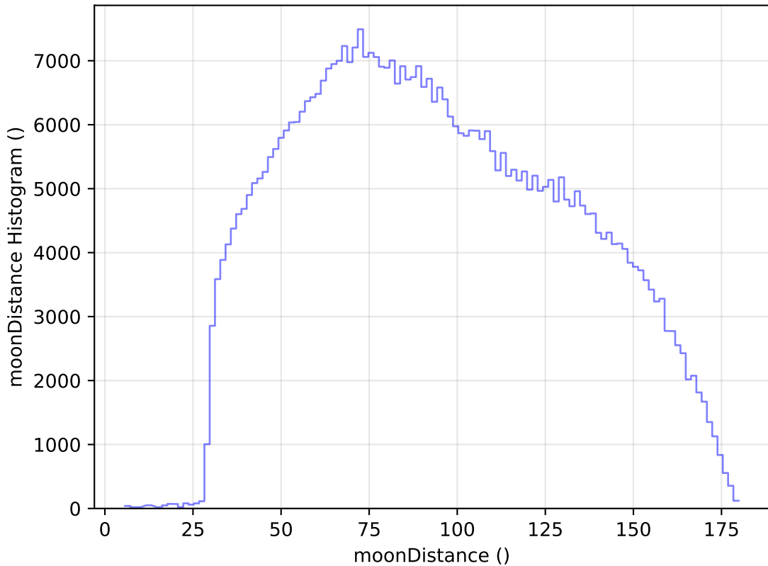
roll_pause_mjdp120_v3.4_10yrs WFD i band: moonDistance Histogram
