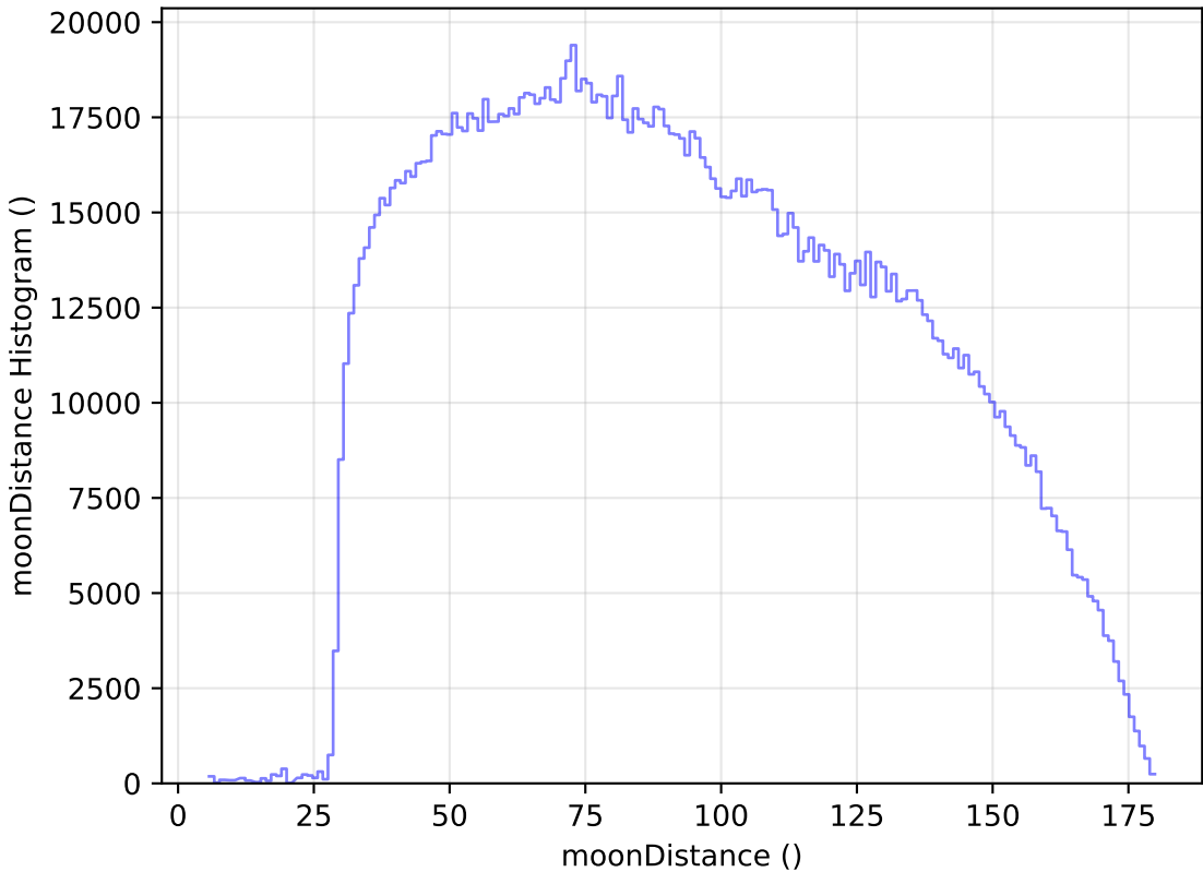
roll_pause_mjdp120_v3.4_10yrs WFD all bands: moonDistance Histogram
