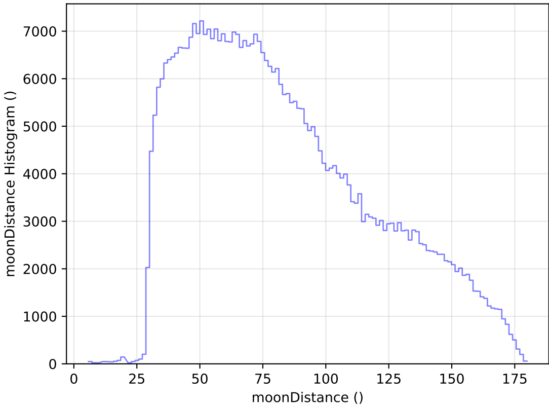
roll_pause_mjdp120_v3.4_10yrs All sky z band: moonDistance Histogram
