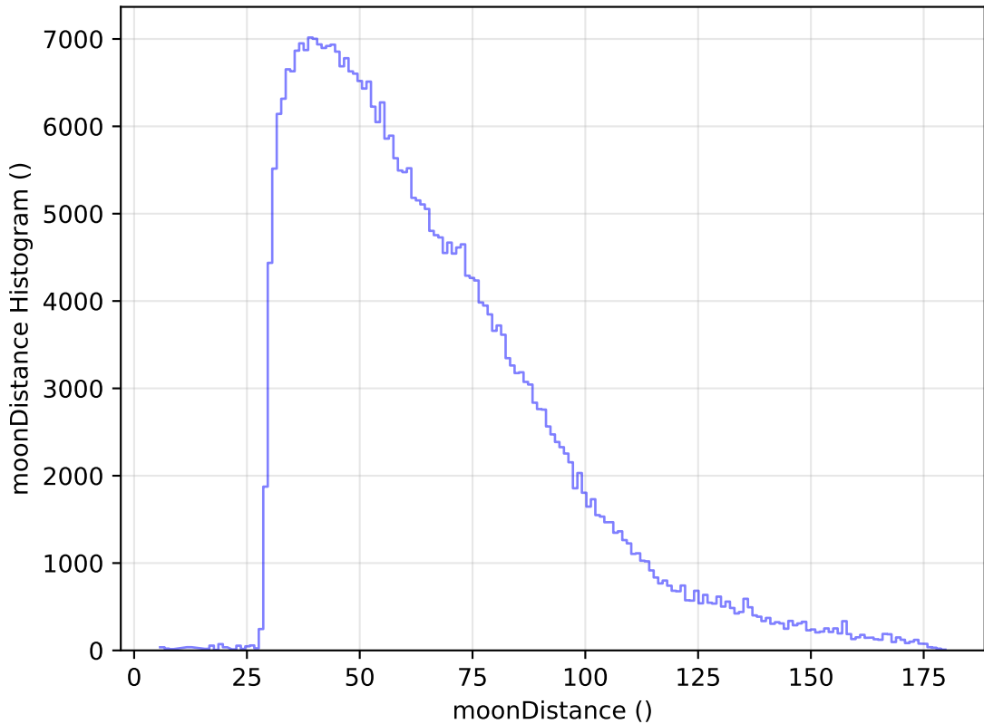
roll_pause_mjdp120_v3.4_10yrs All sky y band: moonDistance Histogram
